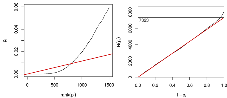
Figure 6: Left: illustration of the Benjamini-Hochberg multiple testing adjustment procedure [2]. The black line shows the p -values ( y -axis) versus their rank ( x -axis), starting with the smallest p -value from the left, then the second smallest, and so on. Only the first 1503 p -values are shown. The red line is a straight line with slope \alpha/n , where n = 8647 is the number of tests, and \alpha = 0.1 is a target false discovery rate (FDR). FDR is controlled at the value \alpha if the genes are selected that lie to the left of the rightmost intersection between the red and black lines: here, this results in 796 genes. Right: Schweder and Spjøtvoll plot, as described in the text.
