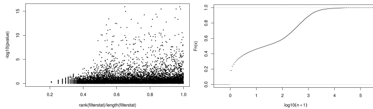
Figure 1: Left: scatterplot of the rank (scaled to [0, 1] ) of the filter criterion filterstat ( x -axis) versus the negative logarithm of the test pvalue ( y -axis). Right: the empirical cumulative distribution function (ECDF) shows the relationships between the values of filterstat and its quantiles.
