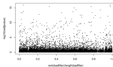
Figure 2: Scatterplot analogous to Figure 1, but with badfilter .
