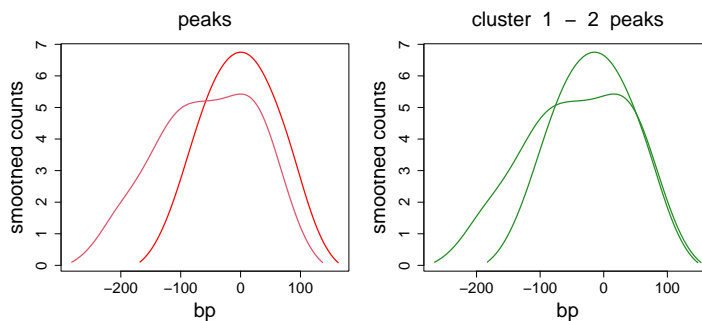
Figure 3: Alignment procedure
