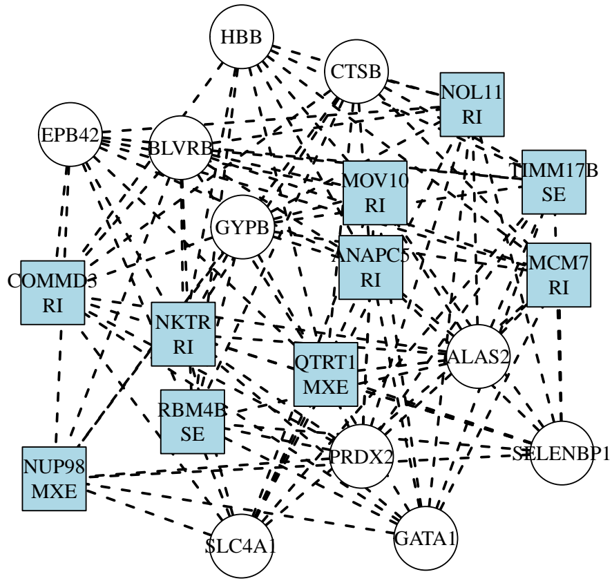
Figure 4: Pathway visualization
