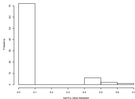
Figure 6: Histogram of the FR statistics p-values mapping cell populations between Sample 1 with Sample 2. The bimodal distribution of the log 10 p-values indicates a clear gap between p-values of matched cell population pairs versus p-values of mismatched cell population pairs.
