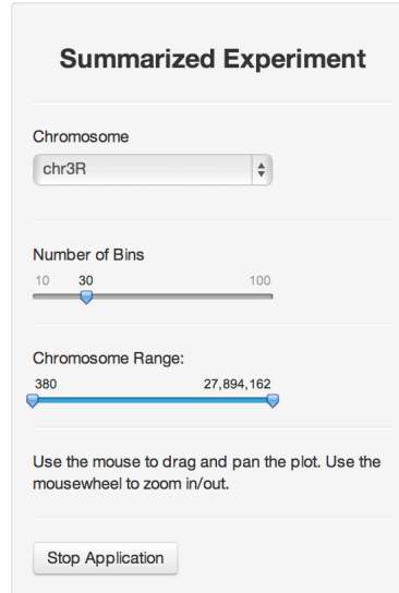
Figure 30: SummarizedExperiment UI
