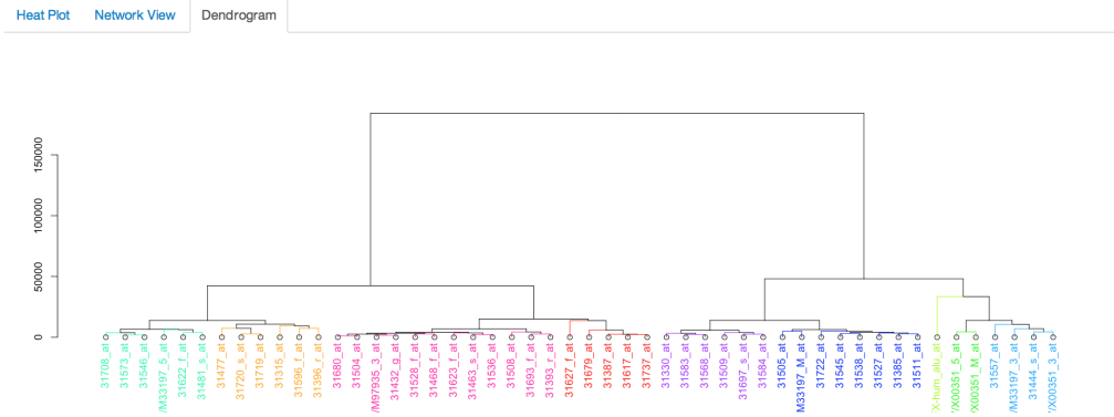
Figure 27: Dendrogram - Probes
